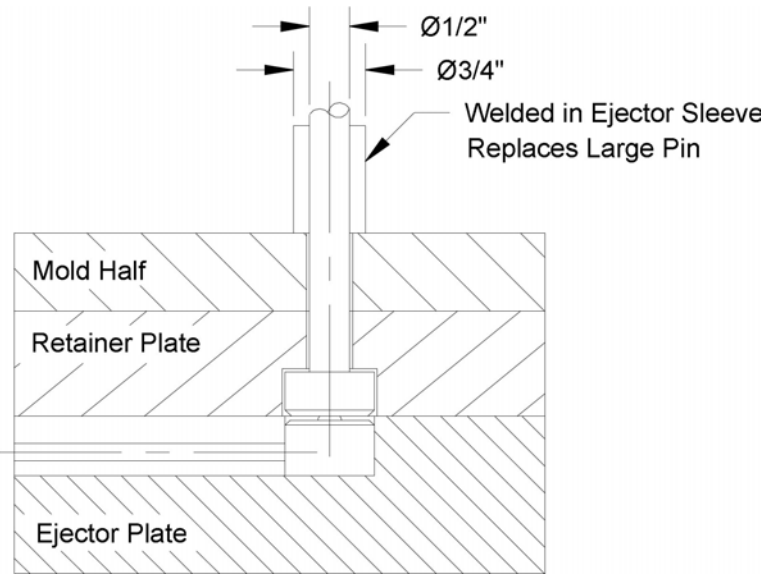
Figure 14: Welded-in Ejector Sleeve Replacement
