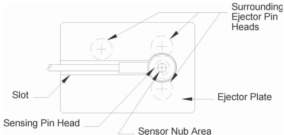
Figure 15: Cutting a Slot Under Interfering Pins
