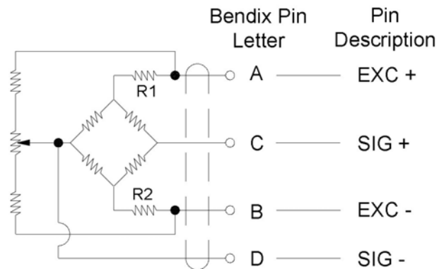
Figure 13: Pin Out Schematic
