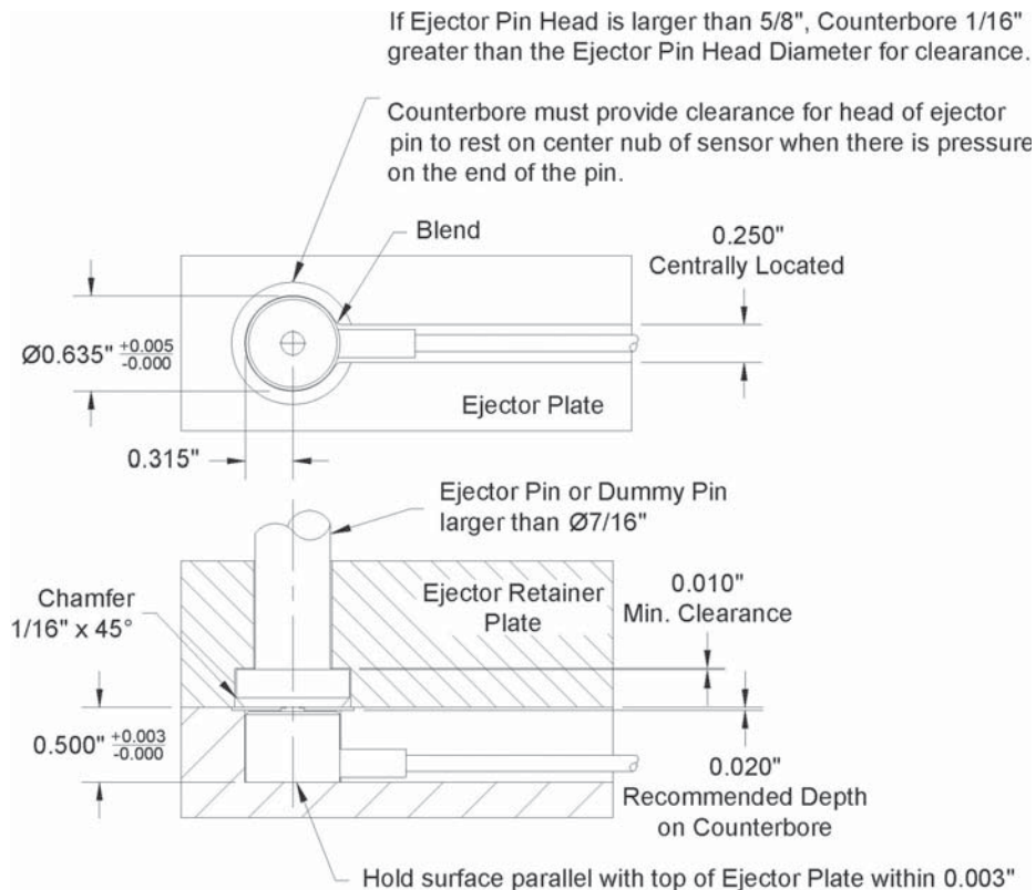
Figure 11: Recommended Mold Cutout for T-445 Sensor
