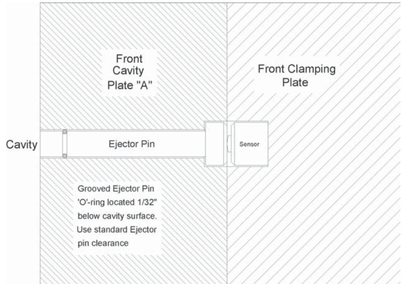
Figure 16: Utilizing Non-Moving Pins
