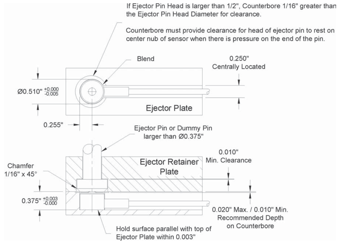
Figure 8: Recommended Mold Cutout for T-412, T-413, & T-414 Sensor
