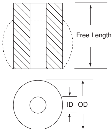
STOCK URETHANE COMPRESSION SPRINGS
